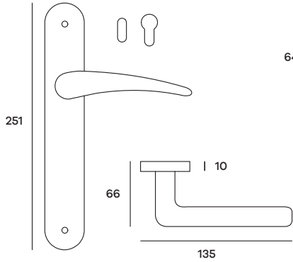
PHEPL05P (Patent) PHEPL05Y (Yale) Maniglia su placca Doorhandle on plate
